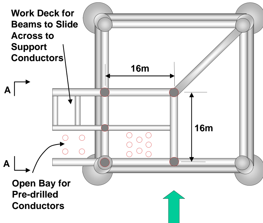
Jack-up Approach to Second Wellbay (90° different to first approach direction)
